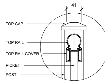
5 DETAIL 1 1:5
