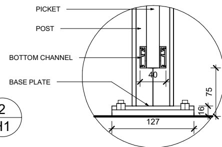
2 DETAIL 2 1:5
