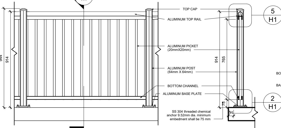
7 FRONT ELEVATION 1:15
