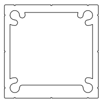
2 Front elevation 1 : 15
