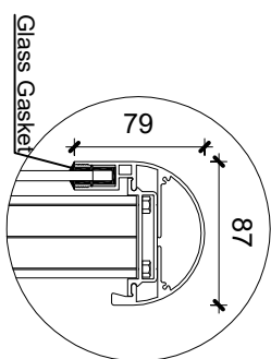
4 Detail 1 1:5
