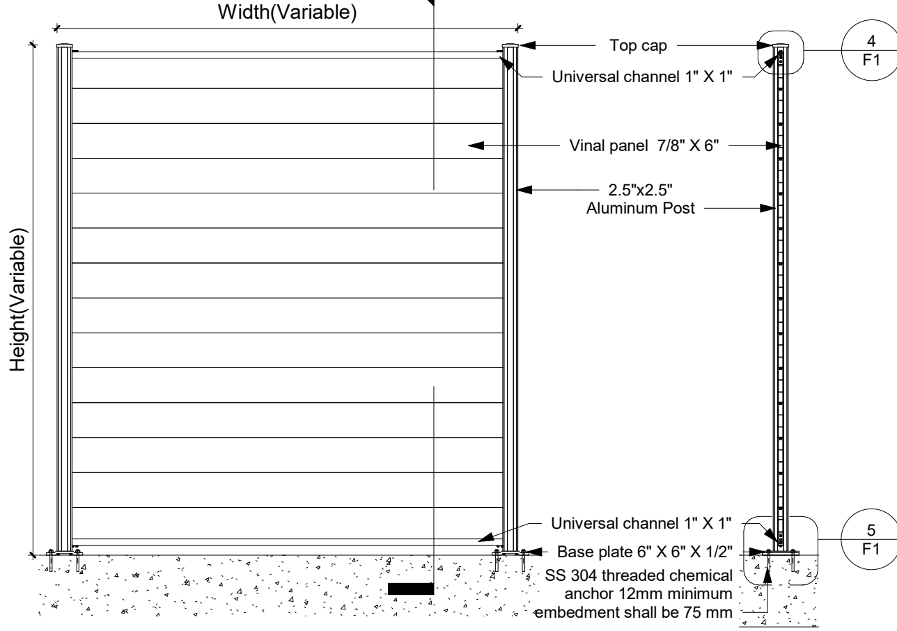
2 Front elevation 1 : 20
